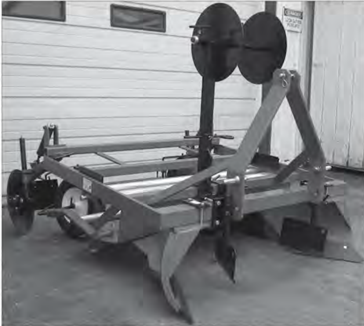
RB448 with Drip Attachment
